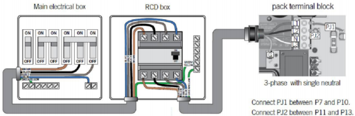
Figure 3. Wiring Schematic for 50 Hz Systems
